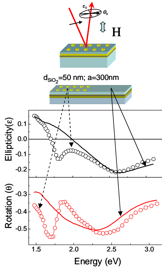
Fig. 3. Kerr rotation and ellipticity spectra, in polar configuration (see upper sketch), for a structure with a nanodiscs array period a = 300 nm and a SiO 2 thickness of 50 nm. The dotted lines correspond to areas of the sample with discs on top of the SiO 2 /trilayer and the continuous lines to areas without Au discs.
