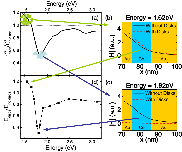
Fig. 7. (a) Non-diagonal element of the reflectivity matrix r_{ps} (magneto-optical contribution), for the structure with array periodicity a = 300 nm and dielectric thickness d_{SiO_2} = 50 nm. (b) Calculated distribution of the electromagnetic field inside the Au/Co/Au continuous trilayer for the system with Au discs on top (red dashed line) and without nanodiscs (black solid line) at energy 1.62 eV (position of the maximum magneto-optical enhancement associated with the presence of the discs, r_{ps}(discs)/r_{ps}(no\ discs) ). (c) Same as in (b) but at energy 1.82 eV (minimum magneto-optical contribution associated with the presence of the discs). (d) Spectral dependence of the ratio of the electromagnetic field inside the Co layer for the continuous SiO 2 /trilayer system with and without nanodiscs on top. (Note: Calculations are done by substituting the Au nanodiscs array layer by an effective medium layer using the Maxwell-Garnett approximation.)
