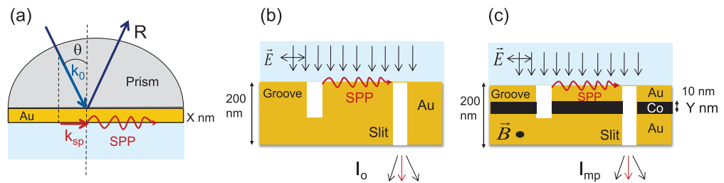
Figure 1. (a) Schematic representation of the traditional SPR configuration. The thickness of the gold layer, X , ranges from 32 to 50 nm depending on the wavelength. (b) Sketch of the plasmonic interferometer. (c) Schema of the MP interferometer. The thickness of the Co layer, Y , depends on the wavelength, varying from 5 to 10 nm.
