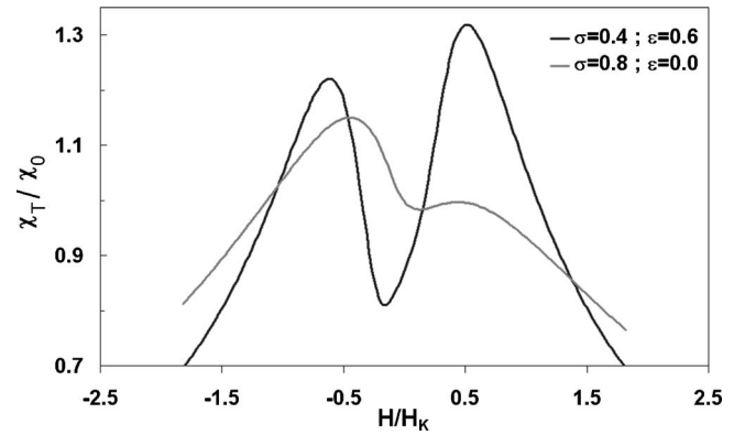
FIG. 7. Theoretically determined \chi_T plots for a randomly oriented nanoparticle system with two different values of the anisotropy field dispersion ( \sigma ) and interparticle interaction ( \varepsilon ) according to the model described in Ref. 13.
